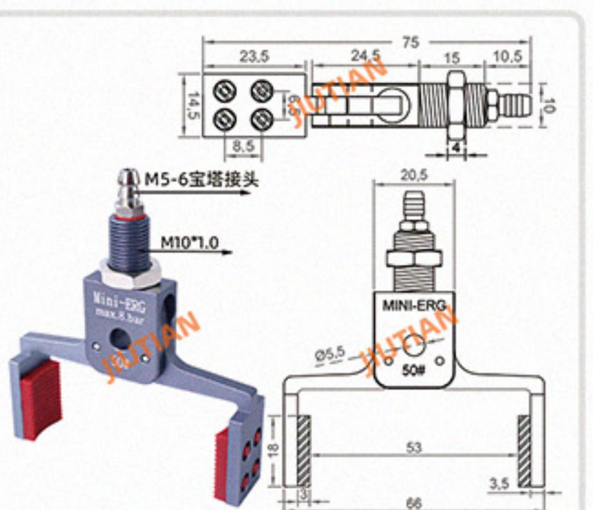
Mini-ERG-50# 夹取范围 36-52MM
