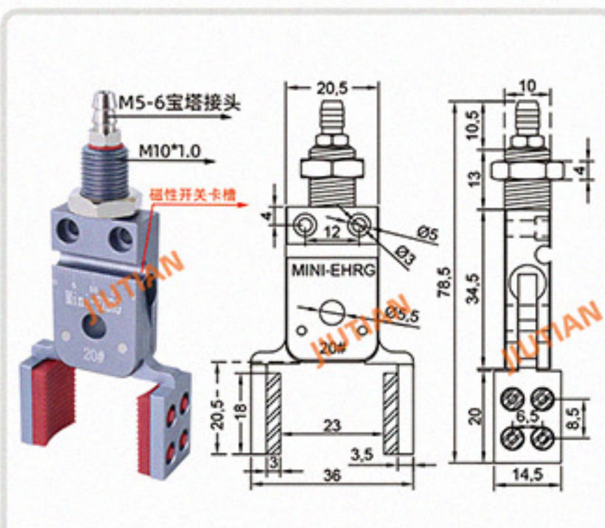
Mini-EHRG-20# 夹取范围 9-22MM
