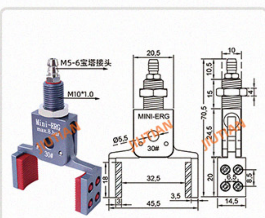
Mini-ERG-30# 夹取范围 18-32MM
