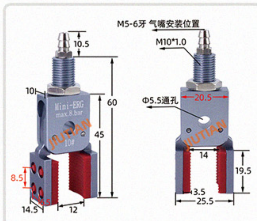
Mini-ERG-10# 夹取范围 0-12MM
