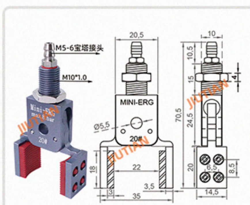
Mini-ERG-20# 夹取范围 8-21MM
