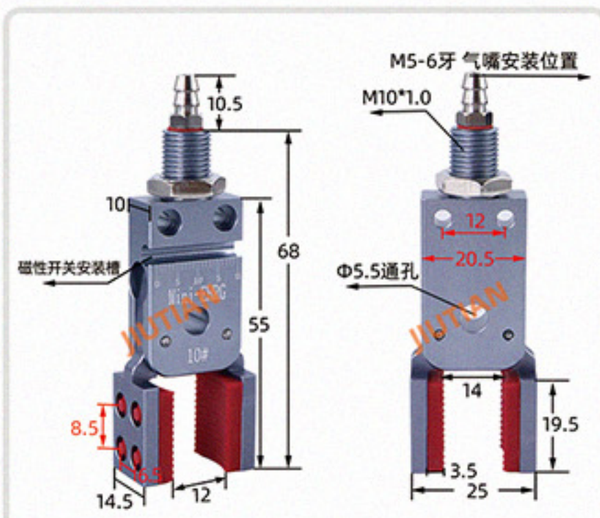
Mini-EHRG-10# 夹取范围 0-12MM
