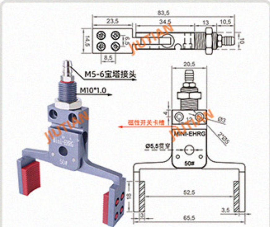
Mini-EHRG-50# 夹取范围 35-52MM
