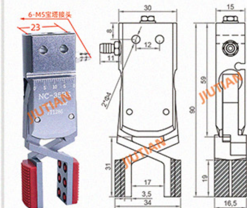
Mini-NC-35BS 夹取范围 34-55mm
