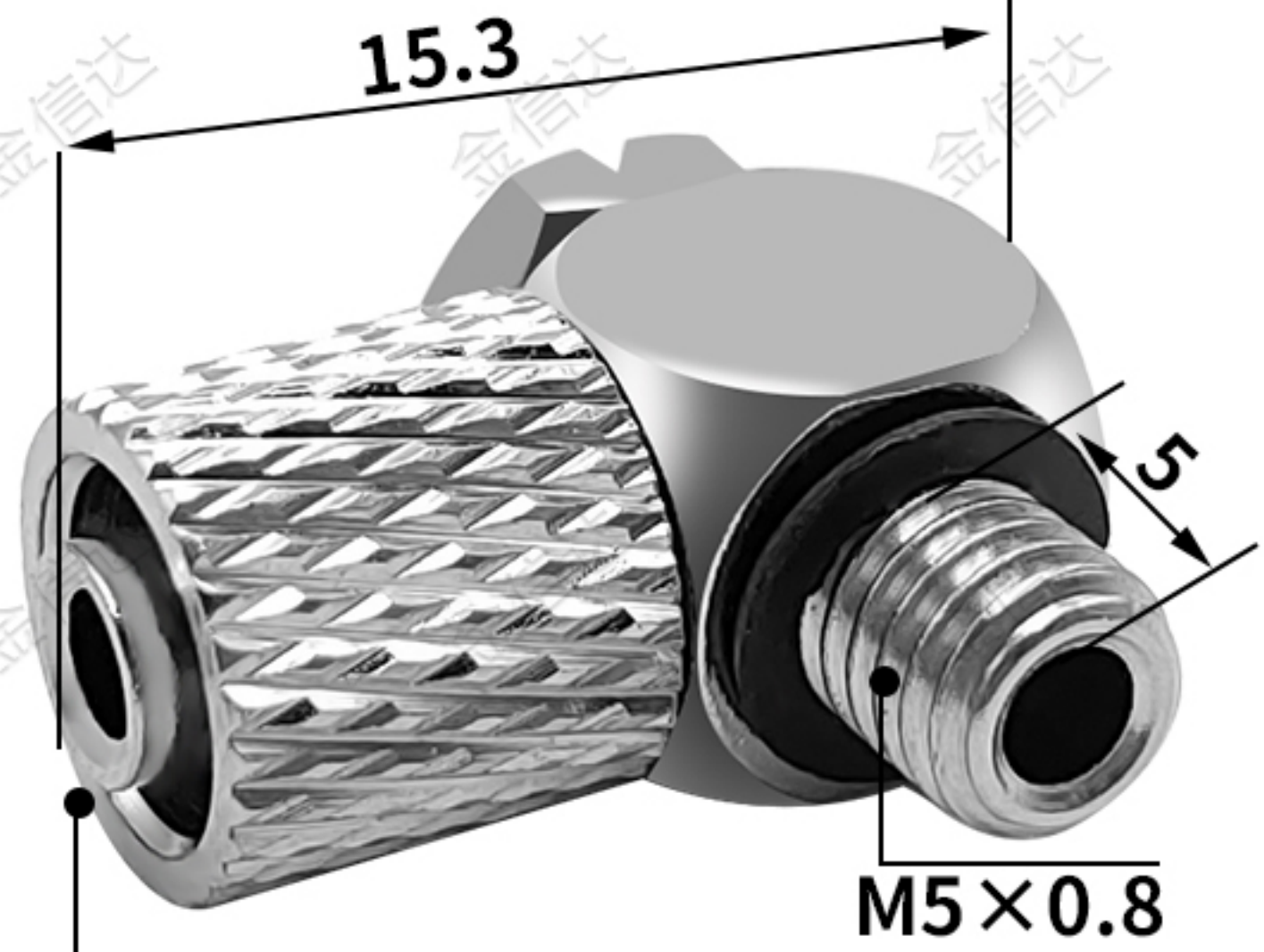
适配接管：6×4 Suitable Tube: 6×4
