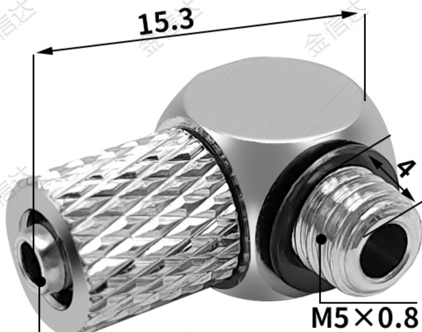
适配接管：3×2 Suitable Tube: 3×2
