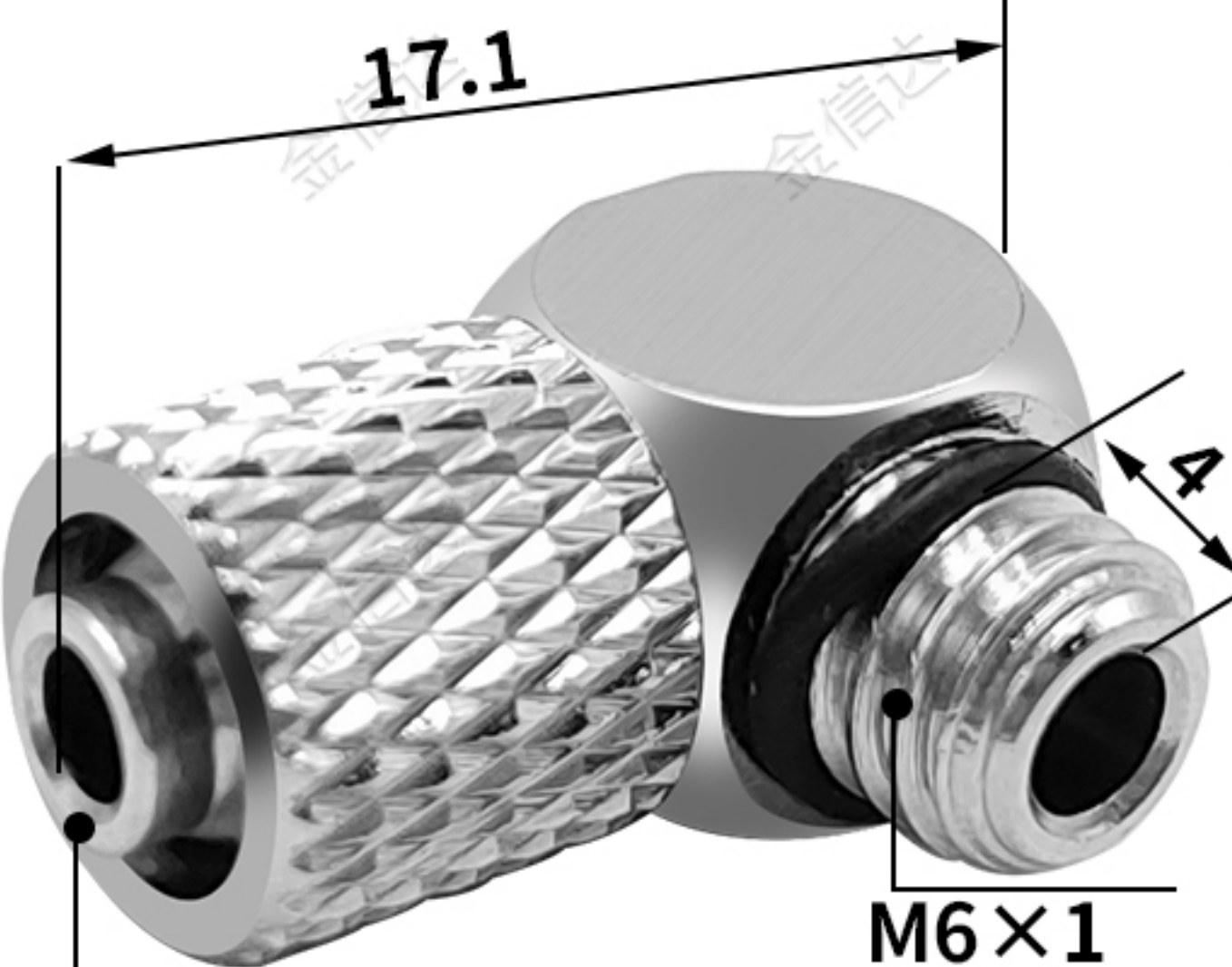
适配接管：6×4 Suitable Tube: 6×4
