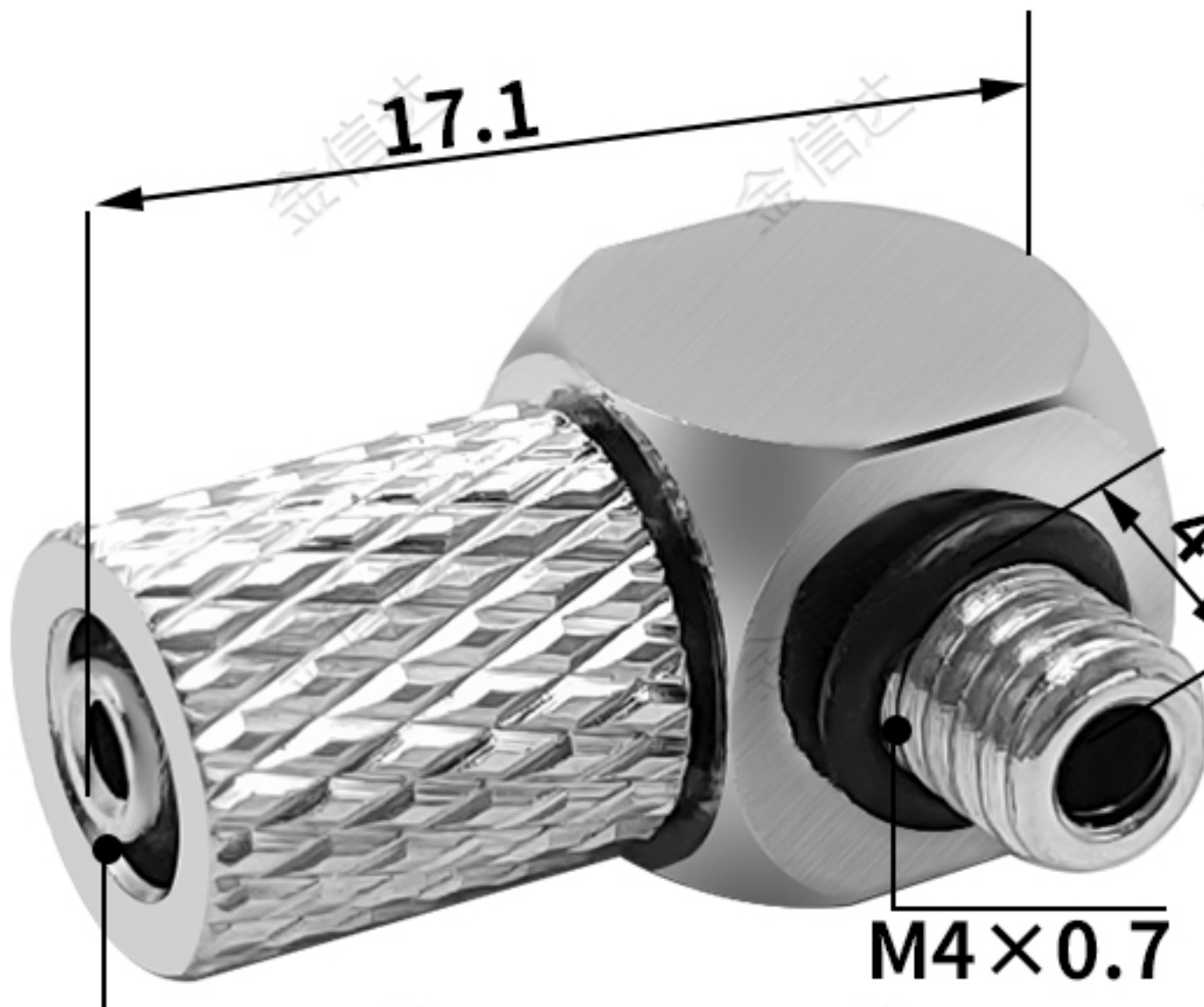
适配接管：6×4 Suitable Tube: 6×4
